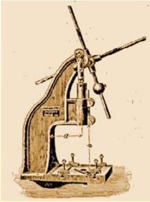
German manual shock press for electric porcelain (1905 La Céramique Industrielle, A. Granger, Ultimheat Museum)
