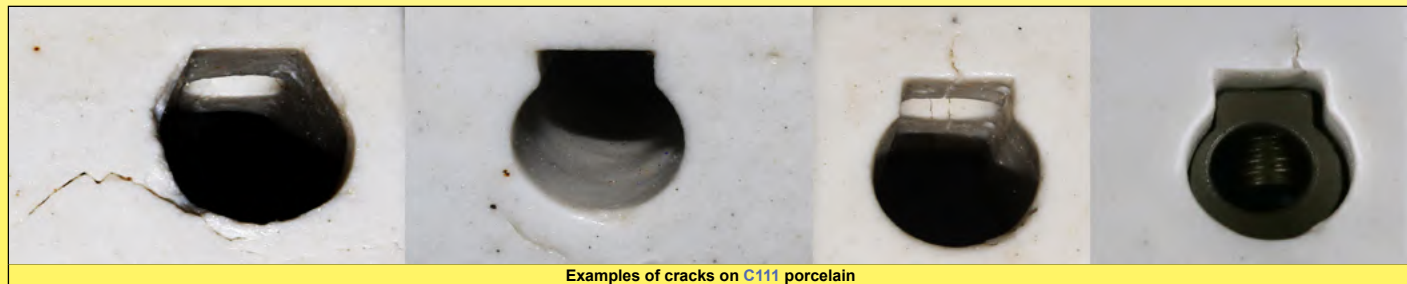
Examples of cracks on C111 porcelain
