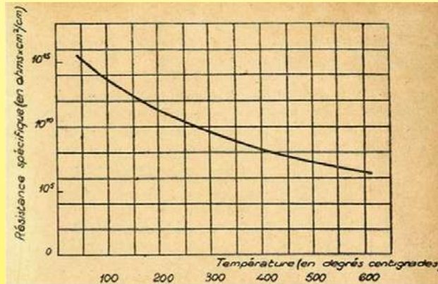
Variation of the specific resistance in ohms.cm/cm² of the porcelain according to the temperature (logarithmic curve). Between 20 ° C and 300 ° C its resistance is divided by 10,000 (1945 Matériaux électrotechniques modernes, Ultimheat Museum)
